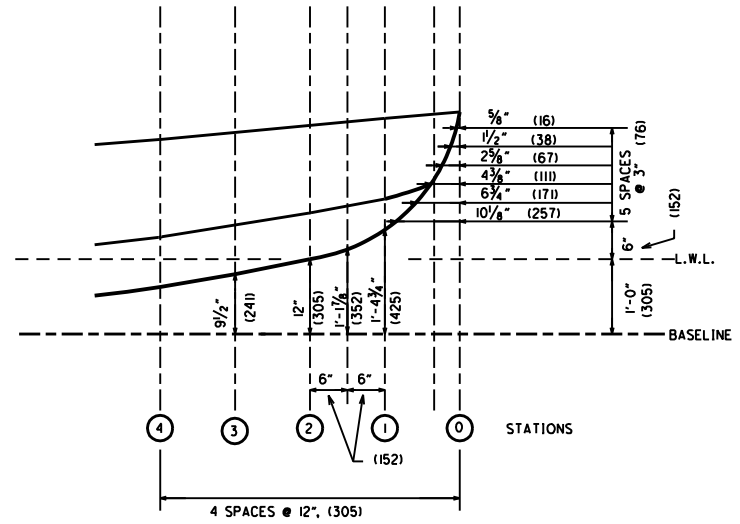
BOW CURVE LAYOUT
